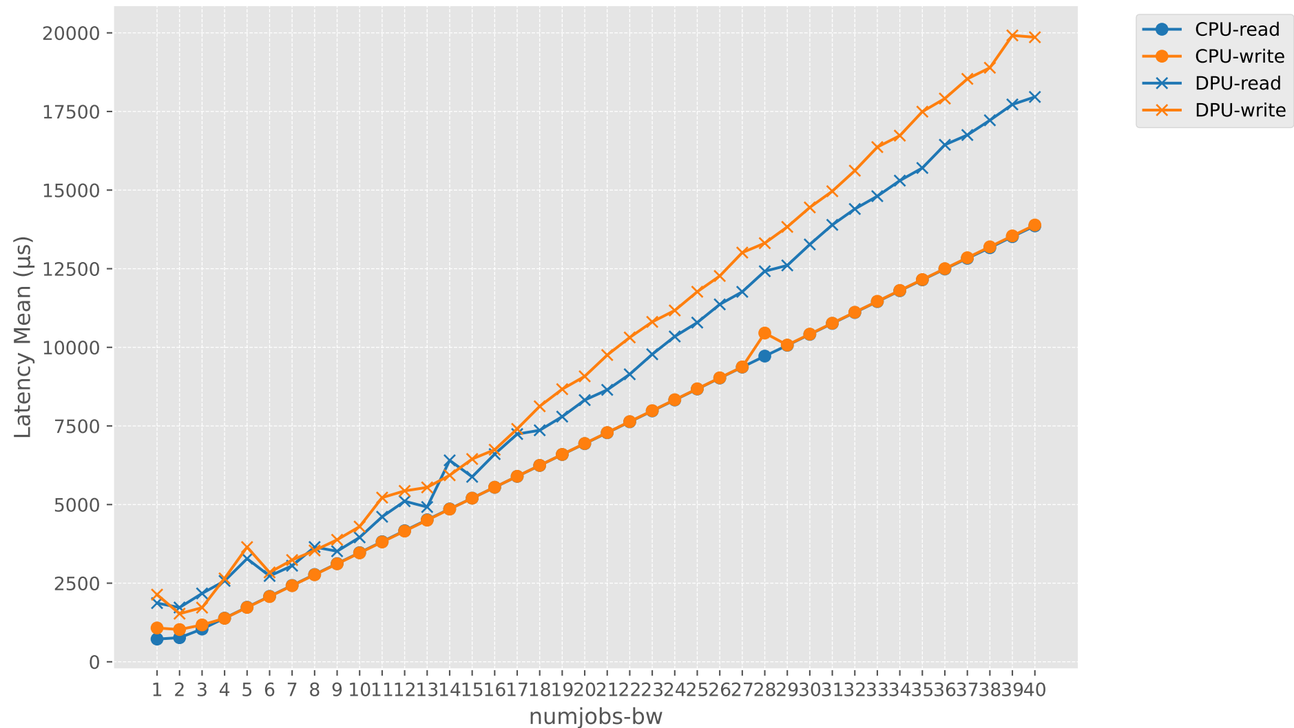
Latency Mean vs numjobs-bw (CPU vs DPU)
